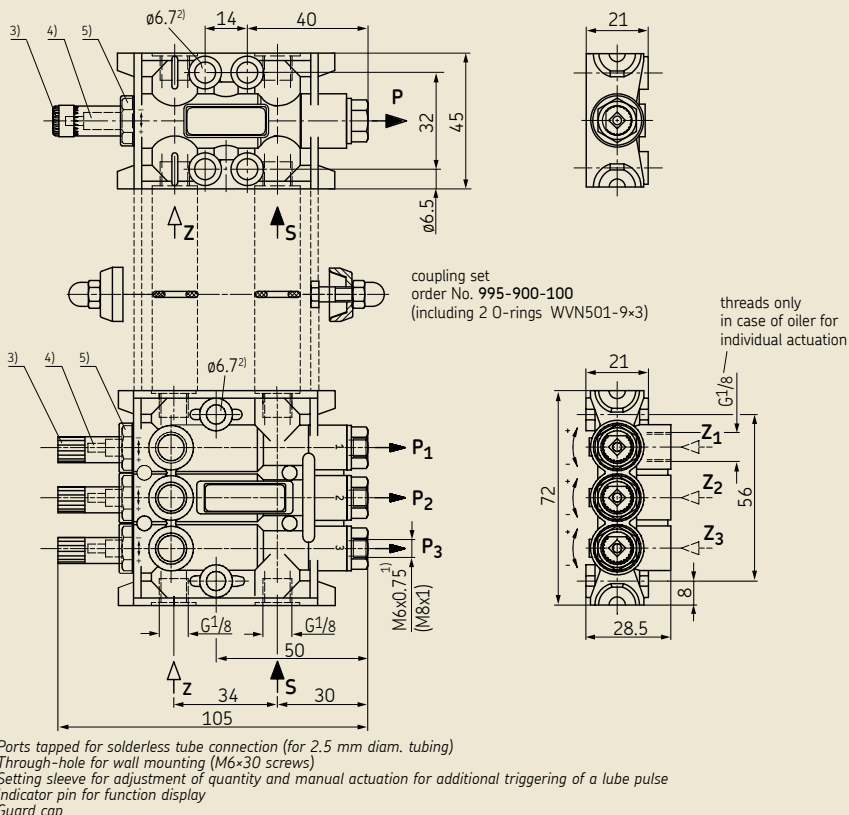
Oiler for group actuation
